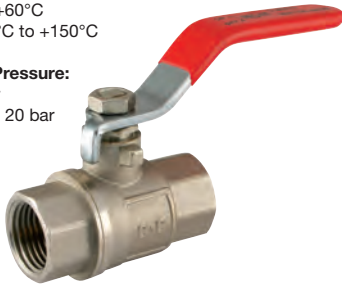
Pro-Fit - Red, Female x Female, BSPP
